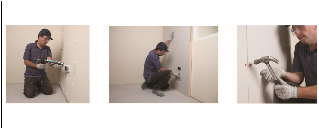
Figure 3 DriLyner DAB (Sealant Variant) installation details
