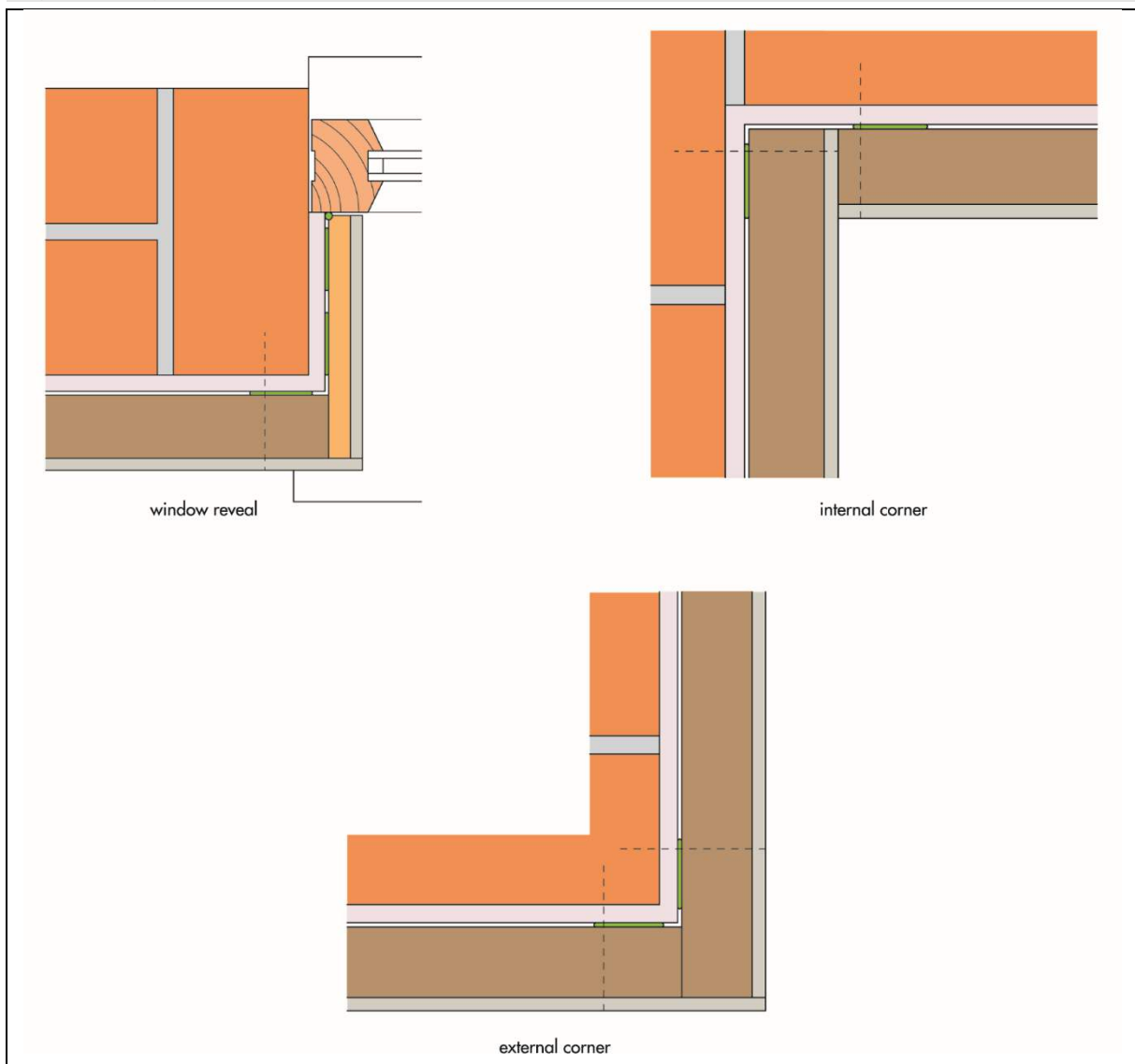
Figure 2 DriLyner DAB (Sealant Variant) construction details
