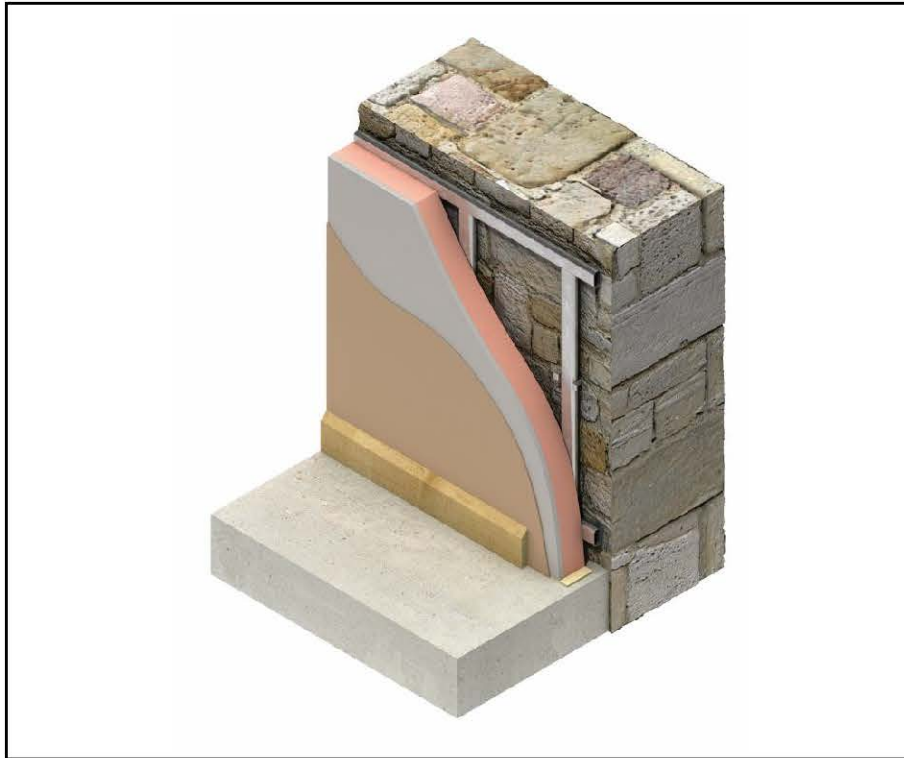
Figure 4 Wetherby internal wall insulation board fixed to metal wall liner
